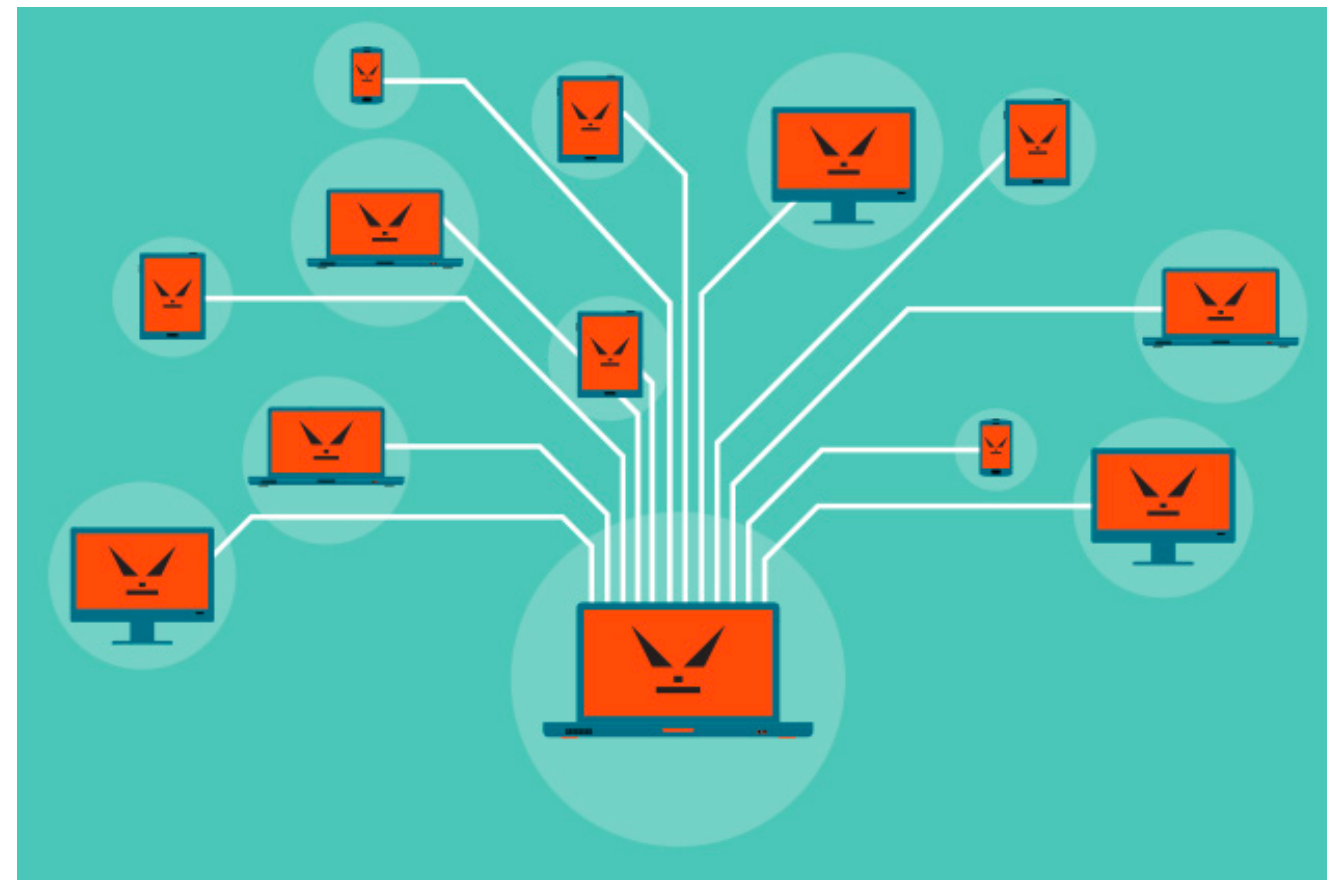
Botnet
